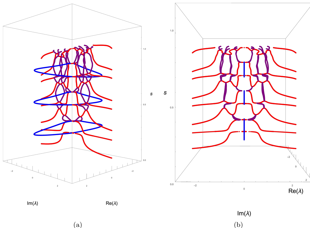
Figure 8. Real (blue), imaginary (red) and complex (purple) eigenvalue curves s^2\lambda \in \text{Spec}(N_s) \cap \mathbb{C} , \lambda \in [-3, 3] \times [-3i, 3i] \subset \mathbb{C} , s \in (0, 1] , under Hypothesis 2.5(i) for a T -periodic stationary state \phi_0 with f(\phi^2) = \phi^2 satisfying \phi'_0(0) = \phi'_0(\ell) = 0 , where \ell = 2T = 13.3854 . Here, \phi_0 is a Jacobi cnoidal function corresponding to an orbit located outside the homoclinic orbit in Fig. 1a. Figures (a) and (b) give two different viewpoints of the same curves. The eigenvalues were computed using Mathematica's NDEigenvalues command.
