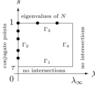
Figure 2. Maslov box in the \lambda s -plane.
