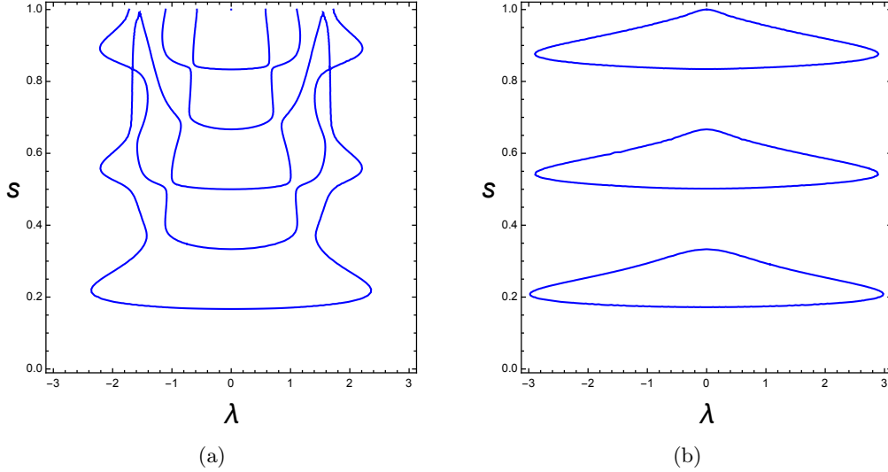
Figure 3. Real eigenvalue curves s^2\lambda \in \text{Spec}(N_s) \cap \mathbb{R} under Hypothesis 2.5(i) associated with a T -periodic stationary state \phi_0 with nonlinearity f(\phi^2) = \phi^2 and \beta = -2 . In (a) \phi_0 is a positive Jacobi dnoidal function (i.e. an orbit located inside the homoclinic orbit in the right half plane in Fig. 1a) satisfying \phi_0'(0) = \phi_0'(\ell) = 0 with \ell = 3T = 9.9398 . In (b) \phi_0 is a Jacobi cnoidal function (i.e. an orbit located outside the homoclinic orbit in Fig. 1a) satisfying \phi_0(0) = \phi_0(\ell) = 0 with \ell = 3T/2 = 10.0391 .
