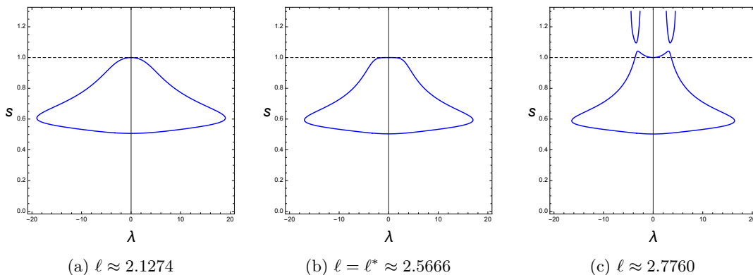
Figure 7. Eigenvalue curves s^2\lambda \in \text{Spec}(N_s) \cap \mathbb{R} under Hypothesis 2.5(i) for T -periodic stationary states \phi_0 satisfying \phi_0(0) = \phi_0(\ell) = 0 , with nonlinearity f(\phi^2) = \phi^6 , \beta = -2 , and domain length \ell = T/2 indicated. These \phi_0 correspond to orbits located outside the homoclinic orbit and in the right half plane of Fig. 1a. (Note the phase plane for (2.9) with f(\phi^2) = \phi^6 is qualitatively similar to Fig. 1a.) Eigenvalues of N are given by intersections with the dashed line at s = 1 . At \ell = \ell^* , we computed \ddot{s}(0) \approx 0 to four decimal places.
