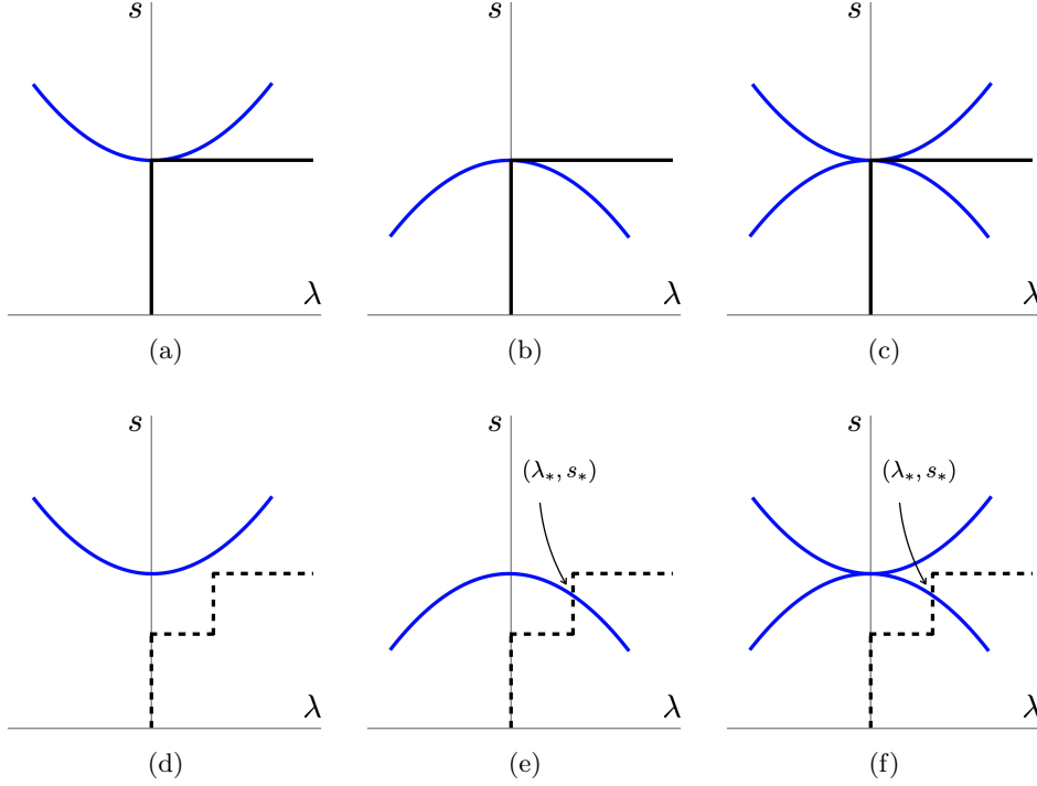
Figure 6. Neighbourhood of the crossing (\lambda_0, s_0) = (0, 1) featuring the eigenvalue curves (parabolas in blue) and the portion of the Maslov box passing through the corner (0, 1) (in black) when (a) \dim \ker(N) = 1 and s^\sharp(0) > 0 , (b) \dim \ker(N) = 1 and s^\sharp(0) < 0 , and (c) \dim \ker(N) = 2 and s_1^\sharp(0)s_2^\sharp(0) < 0 . The path (dashed) to which we homotope the top left corner of the Maslov box in (a), (b) and (c) is given in (d), (e) and (f) respectively.
