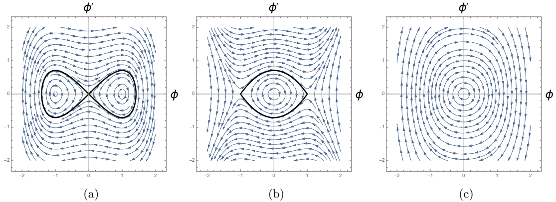
Figure 1. Examples of phase portraits for equation (2.9). In (a) we have cubic focusing nonlinearity f(\phi^2) = \phi^2 and \beta < 0 . The homoclinic orbits in black, representing localised solutions on \mathbb{R} , separate those inside (nonzero Jacobi dnoidal functions) and those outside (Jacobi cnoidal functions that oscillate evenly about \phi = 0 ). In (b) we have cubic defocusing nonlinearity f(\phi^2) = -\phi^2 and \beta > 0 , with periodic orbits existing only inside the heteroclinic cycle in black. In (c) we have f(\phi^2) = \phi^2 and \beta > 0 .
