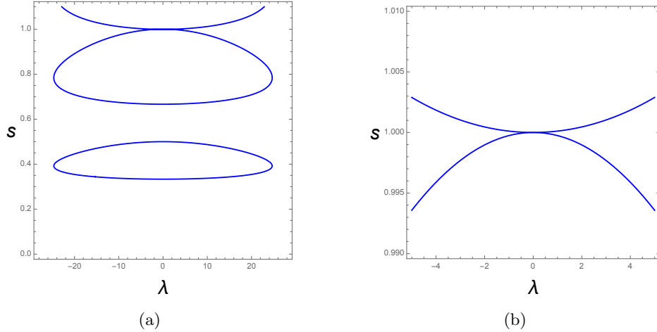
Figure 5. (a) Real eigenvalue curves s^2\lambda \in \text{Spec}(N_s) \cap \mathbb{R} where L_-^s = -\partial_{xx} - 4\pi^2 s^2 , L_+^s = -\partial_{xx} - 9\pi^2 s^2 and \ell = 1 , and (b) a blow-up of the conjugate point (\lambda, s) = (0, 1) .
