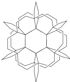
Fig. 2. If the union of the 12 hexagons surrounding A is a Möbius band, then the holonomy around the boundary of A is nontrivial.
